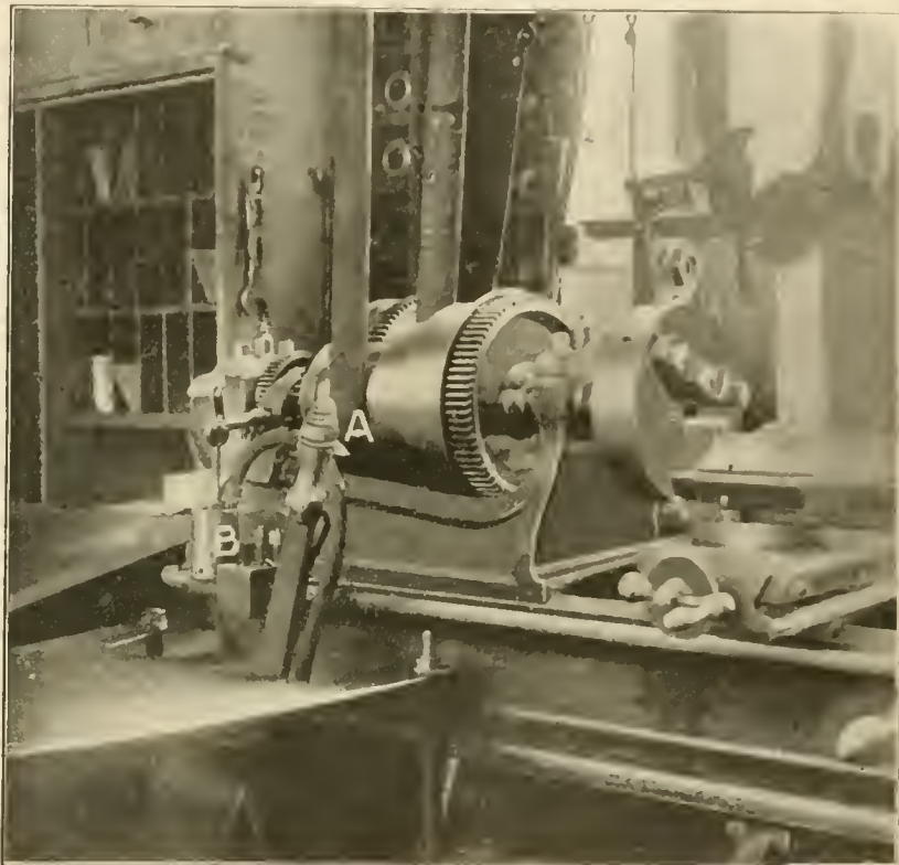
AIR BRAKE ON A BRASS LATHE.
